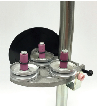
Tensor 3 pivotes desde 0 hasta 3000 dtex Tensioner with 0 pins from 0 to 3000 dtex
